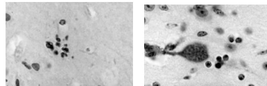
Tachyzoites
