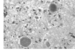
Tissue cysts
