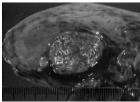
Infected placenta
